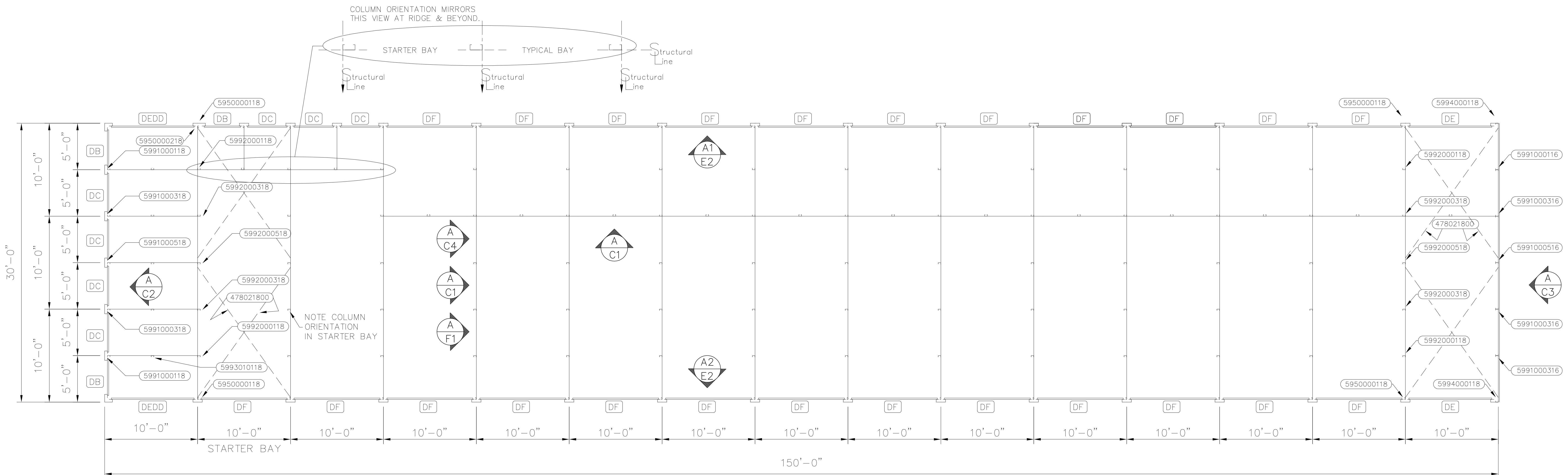
FLOOR PLAN for 30'-0" X 150'-0" MINI STORAGE BUILDING - 1/4:12 PITCH
