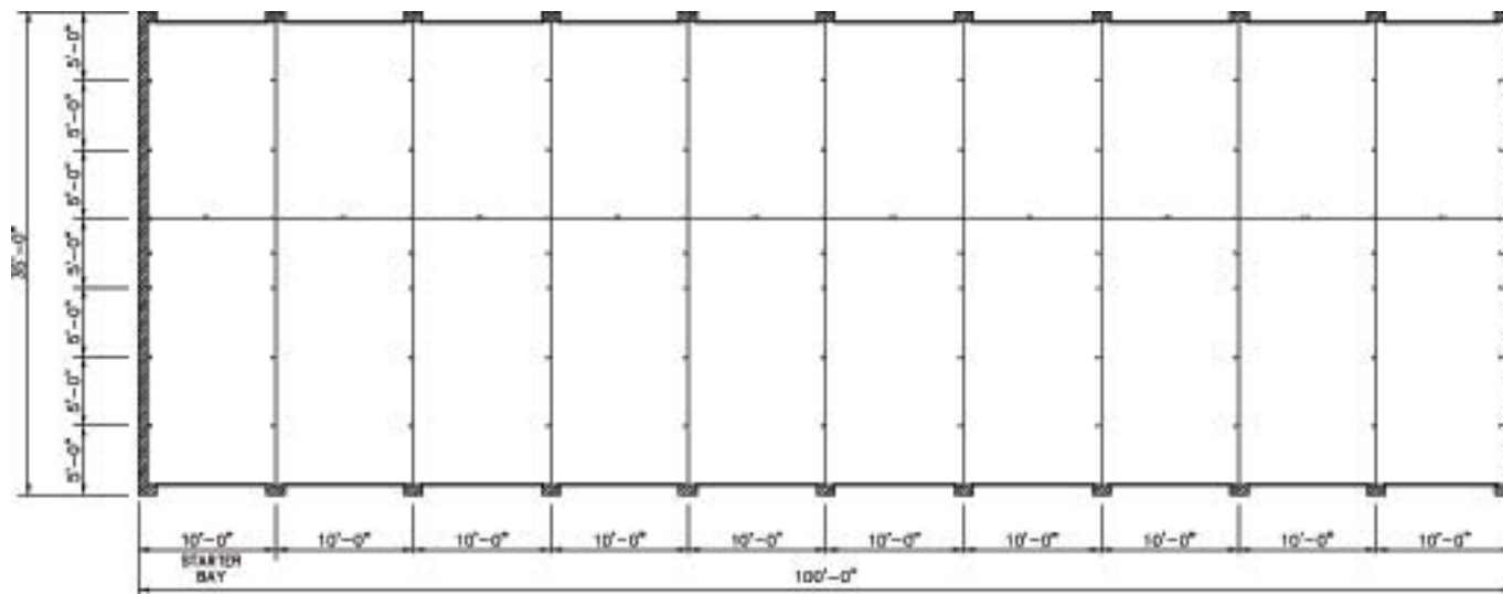
FLOOR PLAN for 35' x 100' BLOCK PERIMETER MINI-STORAGE BUILDING 1/8"=1'-0"
